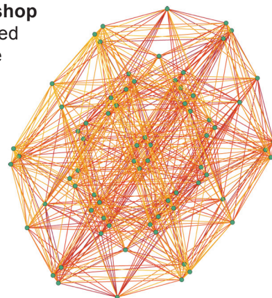
Visualization of The Polytope Associated with the Exceptional Lie Group E6, produced at SAGE Days 9. Photo courtesy of Aurel Meyer.
